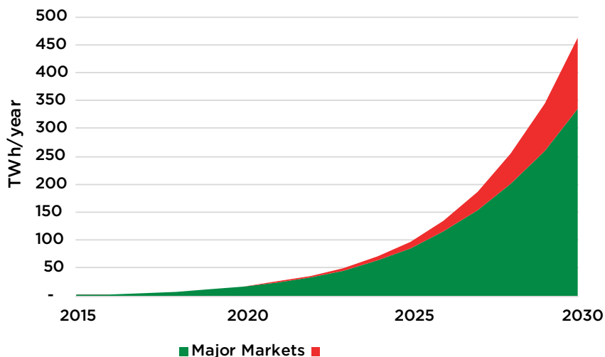
Figure 16: Total electricity demand by electric and plug-in hybrid electric vehicles by region
