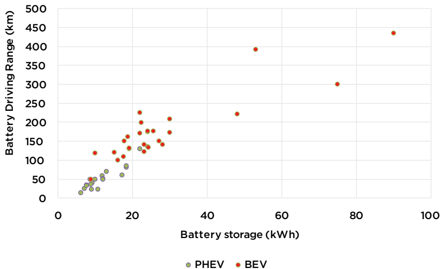
Figure 1: Comparison of battery capacity/driving range for BEVs and PHEVs
