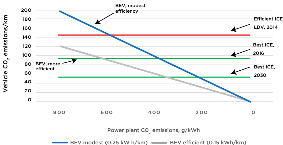
Figure 17: Relation between power plant CO 2 emissions and vehicle efficiency
