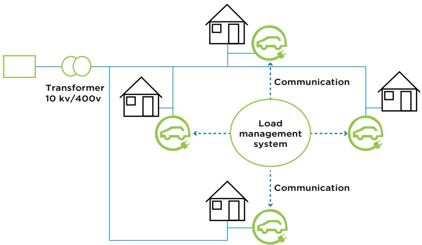
Figure 11: A diagram shows the concept of a load management system
