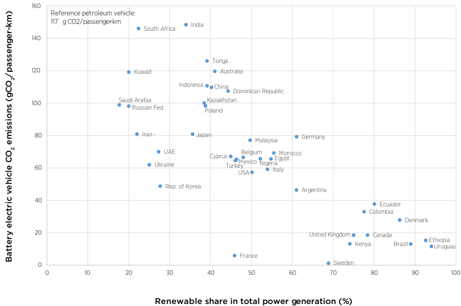
Figure 18: Relation between renewable energy share in total power generation and the electric vehicle CO 2 emissions, IRENA projection for 2030
