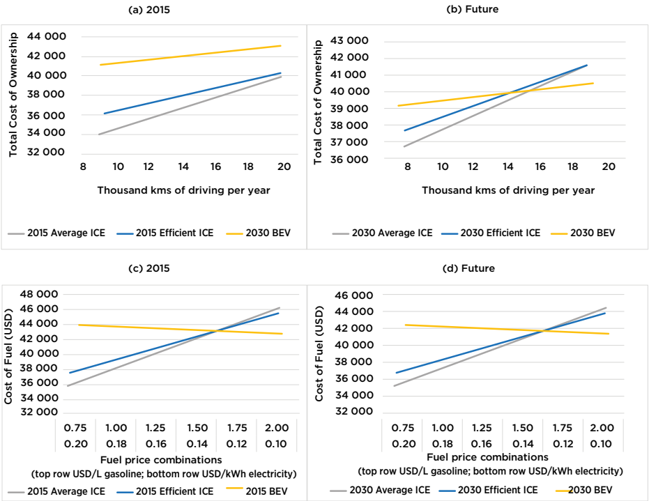
Figure 7: Conventional ICE, Efficient ICE, and EV life-cycle cost comparison by: (a) driving levels per year, 2015, (b) driving levels per year, 2030, (c) combinations of fuel prices, 2015, (d) combinations of fuel prices, 2030
