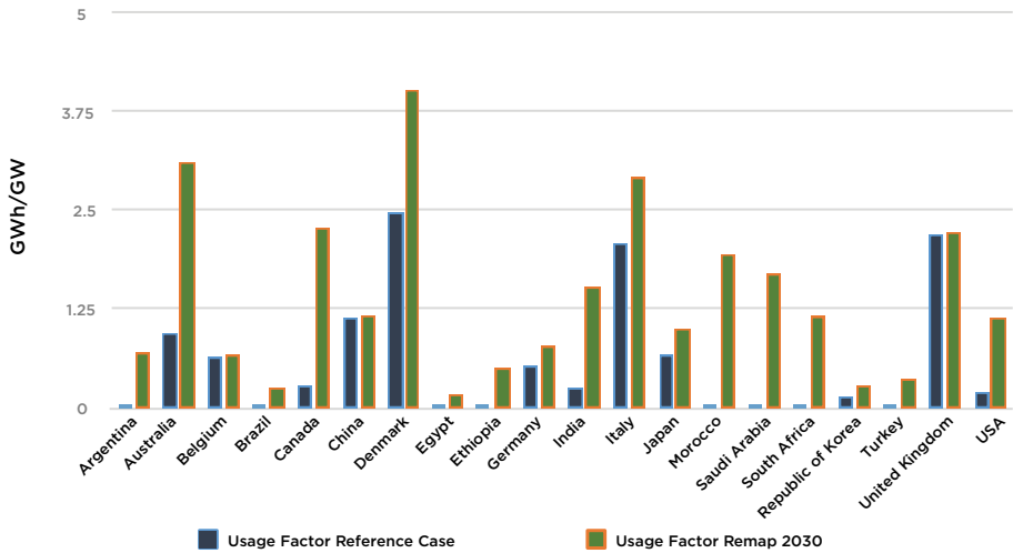
Figure 9: The usage factor of EV's battery storage capacity with respect to the VREs installed capacity
