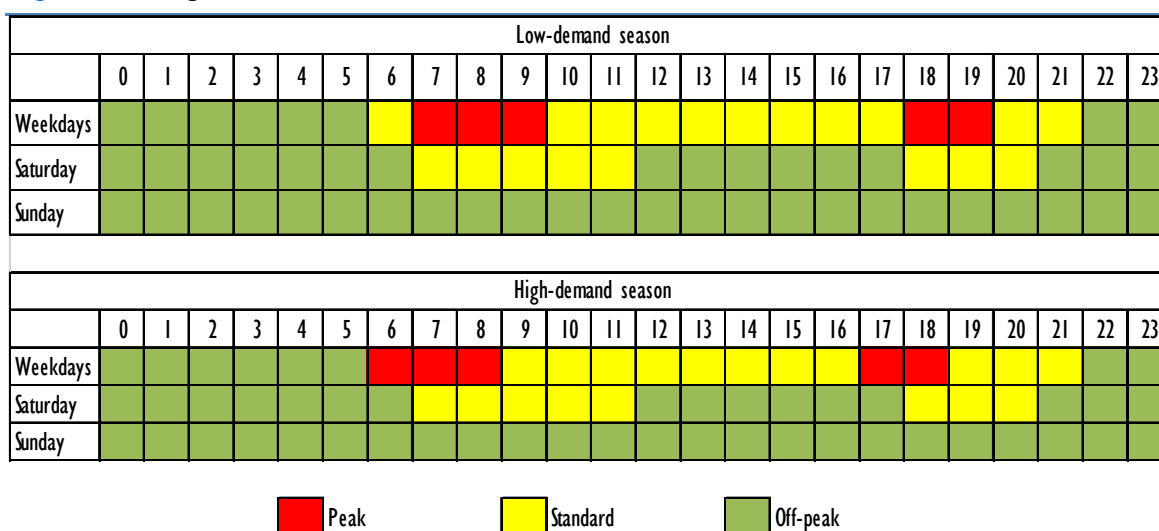
Figure 6.6 • Megaflex tariff hours structure
